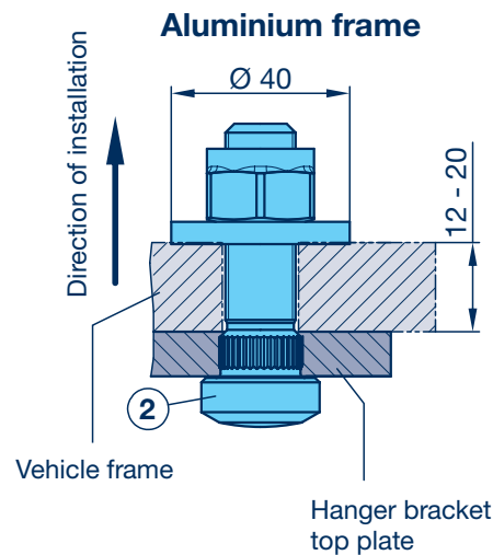
Knurled screw M 16, connection frame / hanger bracket
