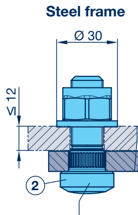
Knurled screw M 16, connection frame / hanger bracket
