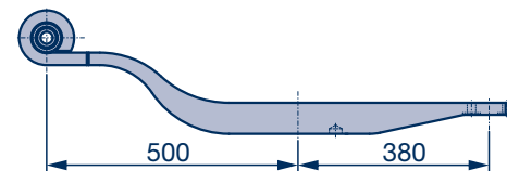
Trailing arm, series ALUW for optimised position of brake cylinder and axle lift
