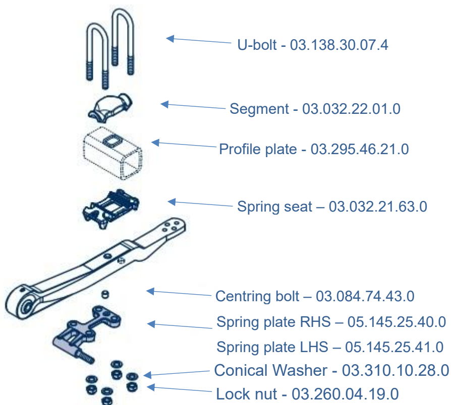
Figure 4 - ALU suspension
